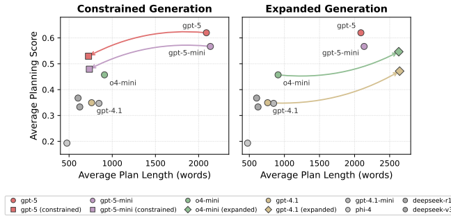
Figure 3: Relationship between plan length and Average Planning Score under constrained and expanded generation settings. Left: When response length is controlled, GPT-5 and GPT-5-mini generate shorter plans but remain the top performers. Right: When longer outputs are allowed, GPT-4.1 and o4-mini produce more extensive plans with higher scores. Arrows indicate the shift from the original to the constrained or expanded setting.
