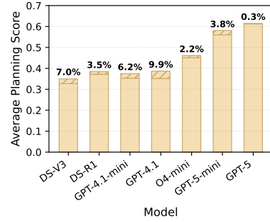
Figure 4: Impact of curated literature on average Planning Score across LLMs. Bars show baseline performance (solid) and the improvement with curated literature (hatched). DS denotes DeepSeek.
